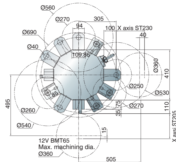
12V BMT65 tool
