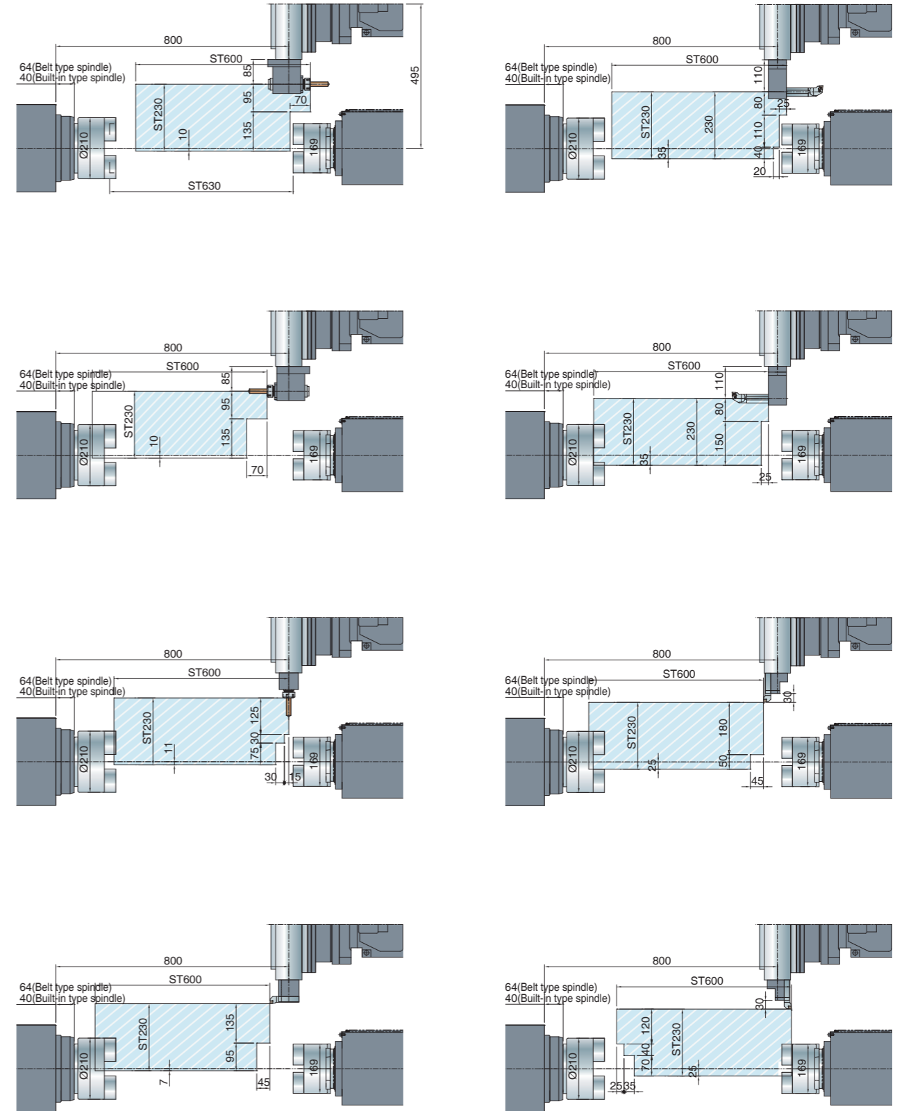
TD-2000YB(C) 16V/VDI-30 tool
