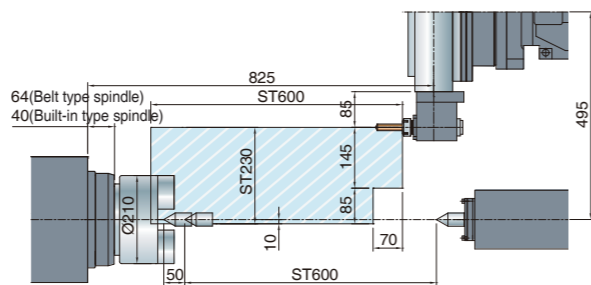
TD-2000Y 16V/VDI-30 tool
