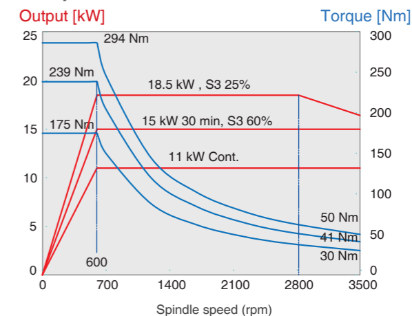
Built-in type sub-spindle motor
