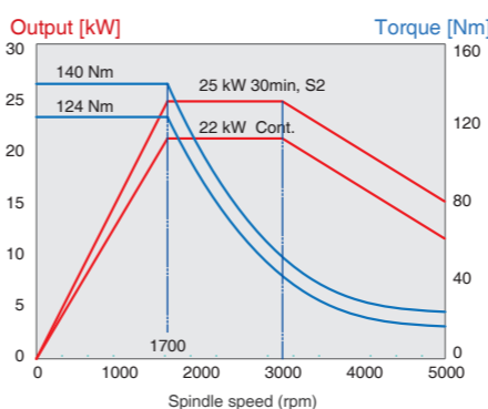
TD-2500Y Built-in type spindle motor (Opt.)
