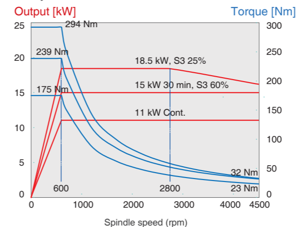
TD-2000Y Built-in type spindle motor (Opt.)
