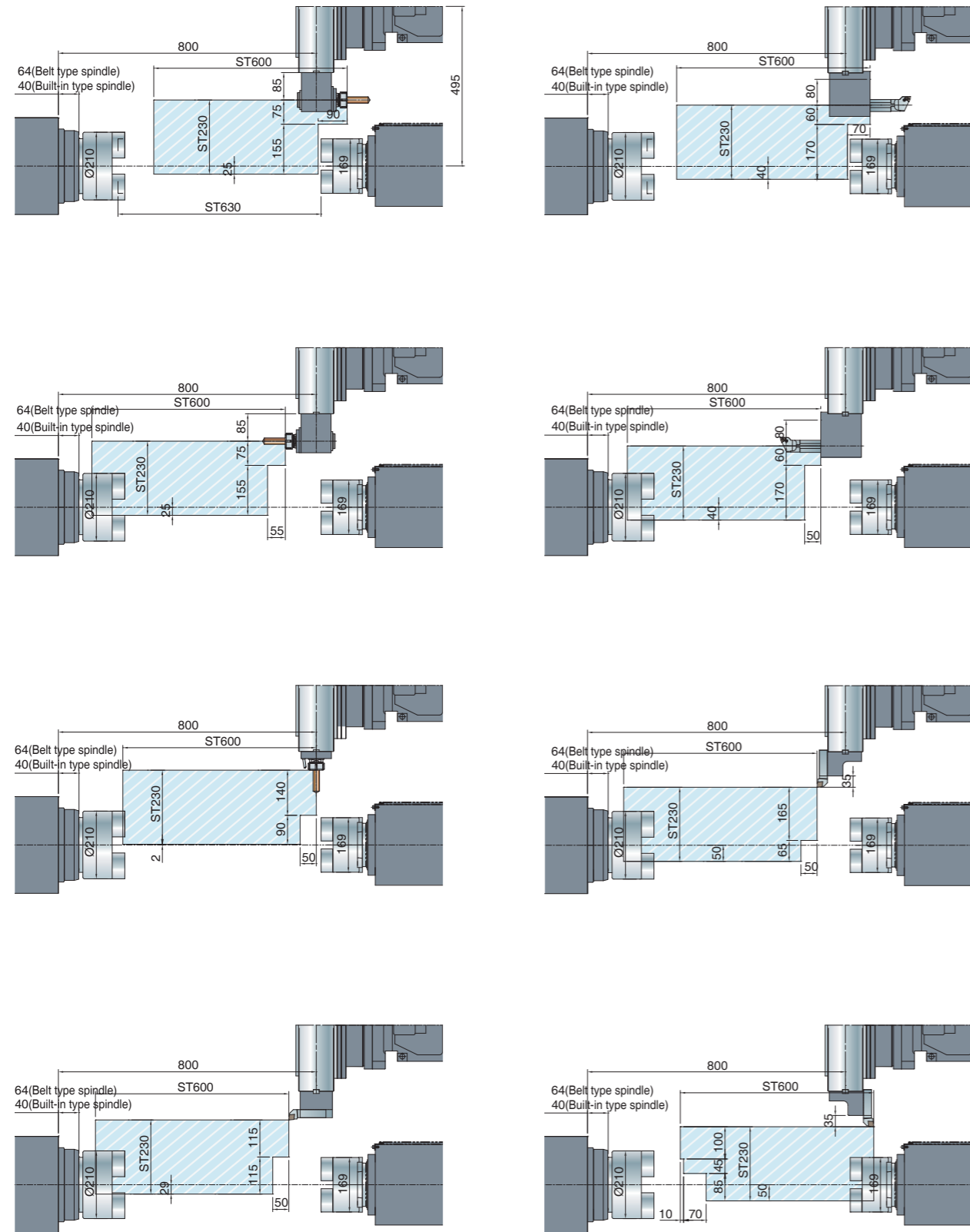
TD-2000YB(C) 12V/BMT-65 tool
