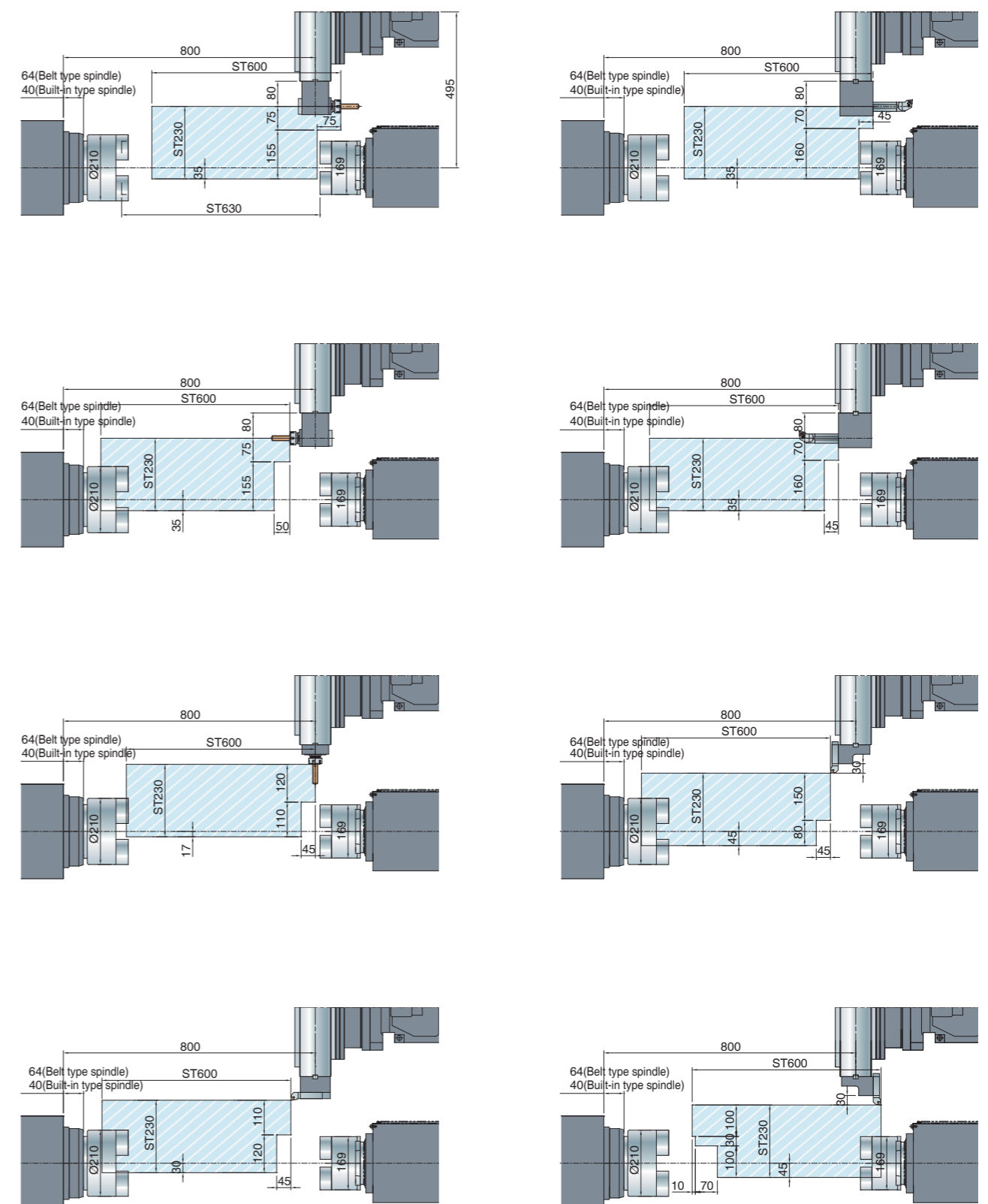
TD-2000YB(C) 16V/BMT-55 tool
