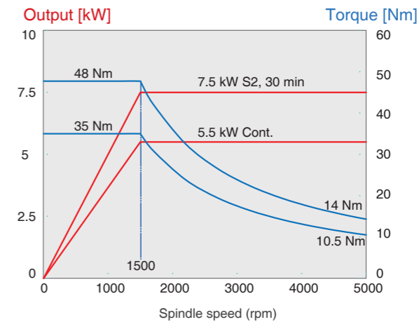
TD-2500Y Built-in type spindle motor (Opt.)
