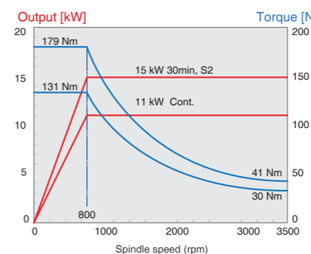
TD-2500Y Built-in type spindle motor (Opt.)
