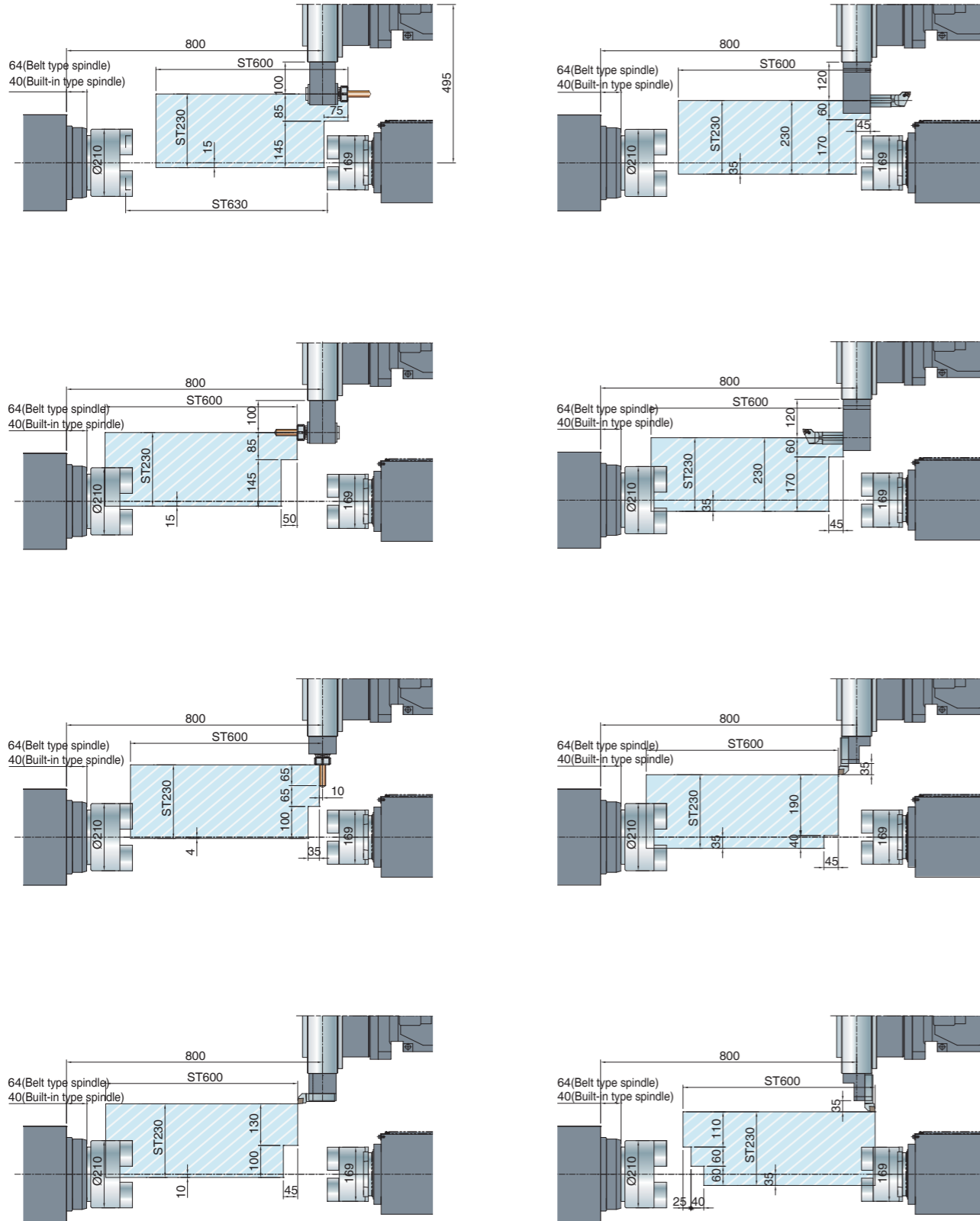
TD-2000YB(C) 12V/VDI-40 tool
